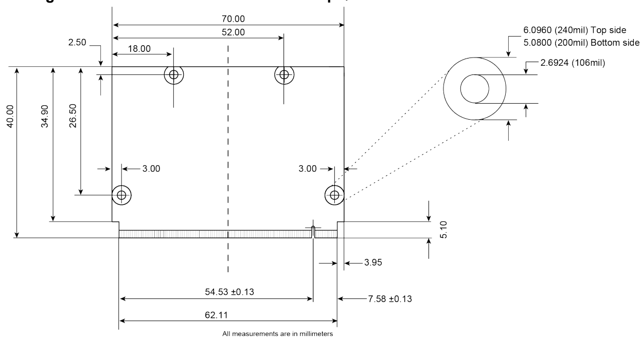
Figure 1-4: Mechanical Dimension of the \mu Qseven Module
