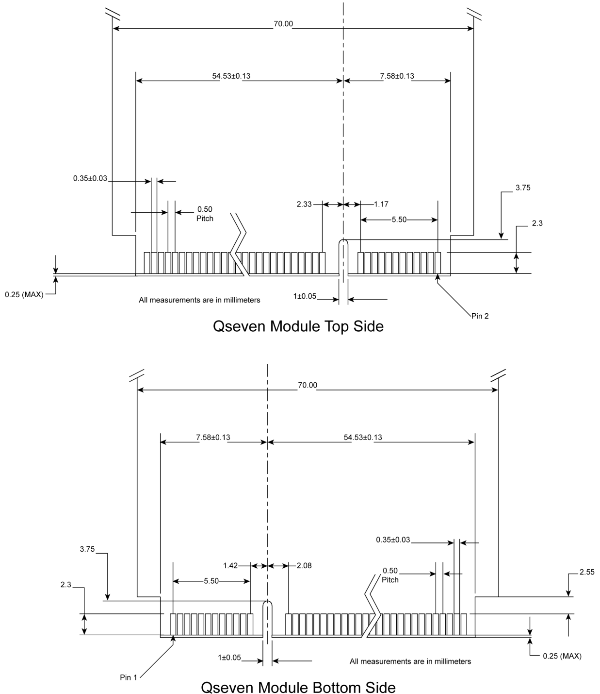
Figure 1-5 Edge Connector Dimensions of the Qseven® Module
