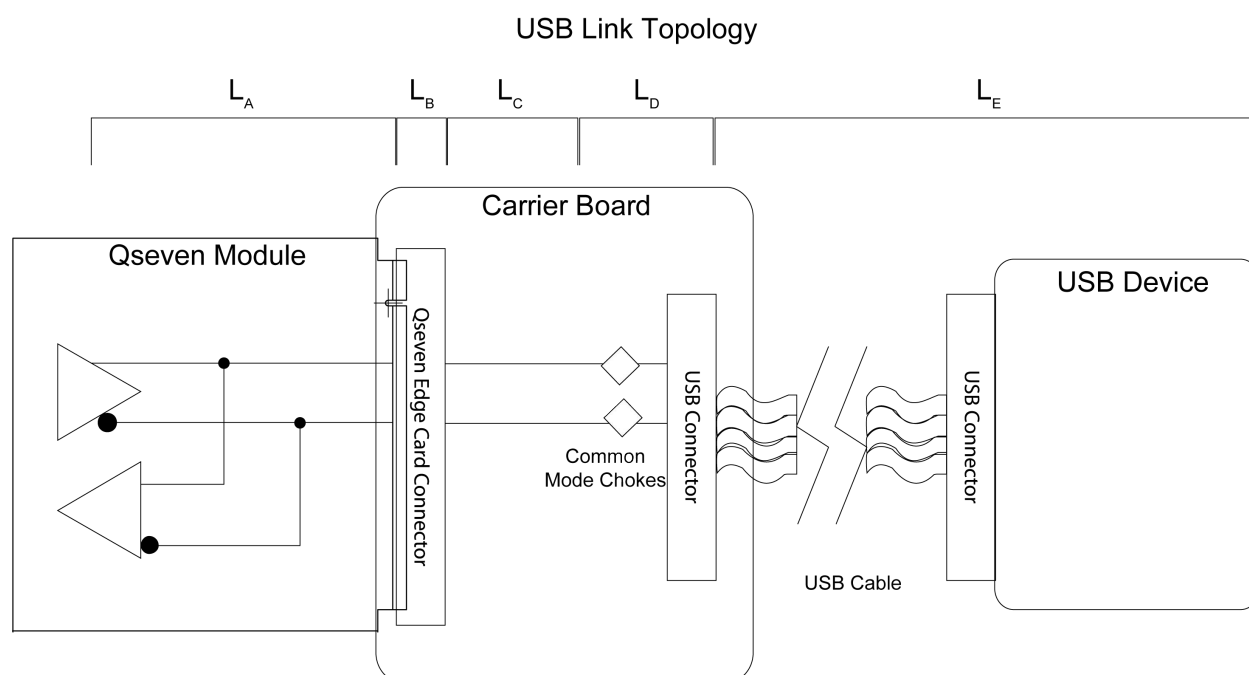
Figure 4-5 USB 2.0 Link Topology
